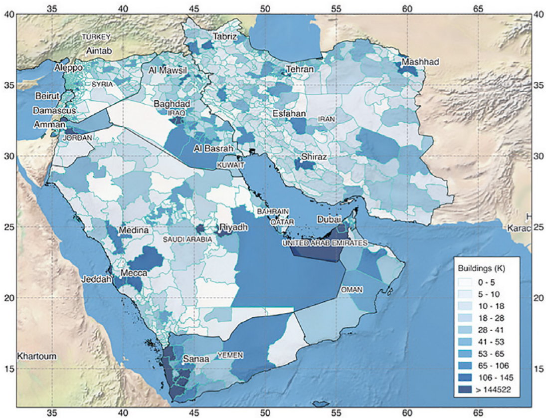
Figure 3.24. Distribution of number of residential buildings at the smallest available administrative subdivision for 12 countries in the Middle East as of 2018
